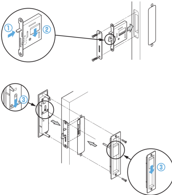
Privacy (PRV) Indicator (IND) Cylinder Lock (CLD) Double sided slide (DSL)
